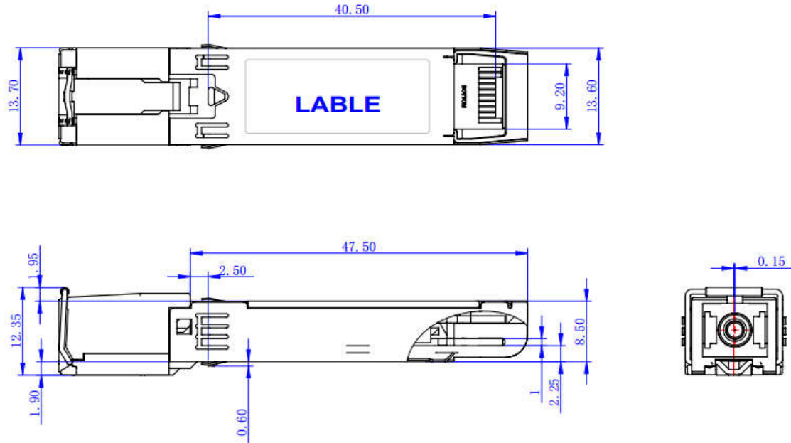
Figure8 Package Outline for MPLO20-D6C-B4T1
