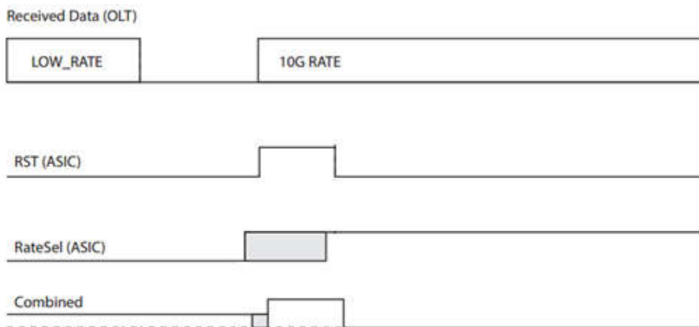
3-level signaling recommended sequence
