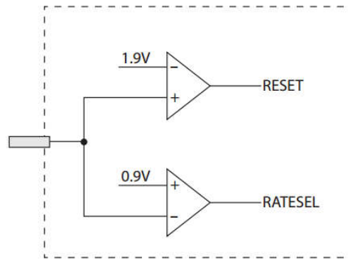
3-level signaling logic
