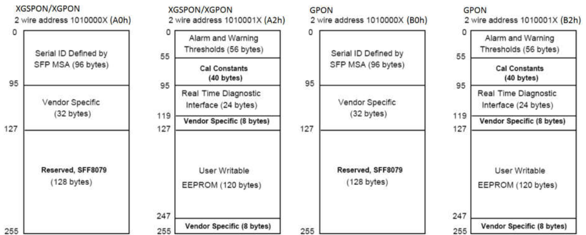
Figure 7 EEPROM Memory Map Specific Data Field Descriptions
