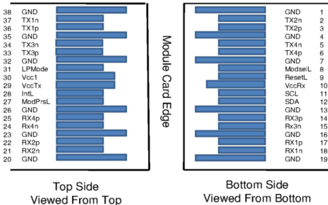
Figure 1 Pinout of Connector Block on Host Board
