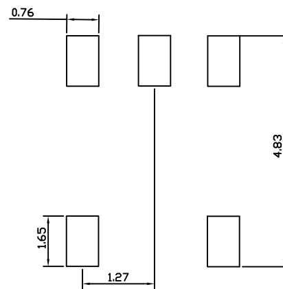
Recommend PAD layout
